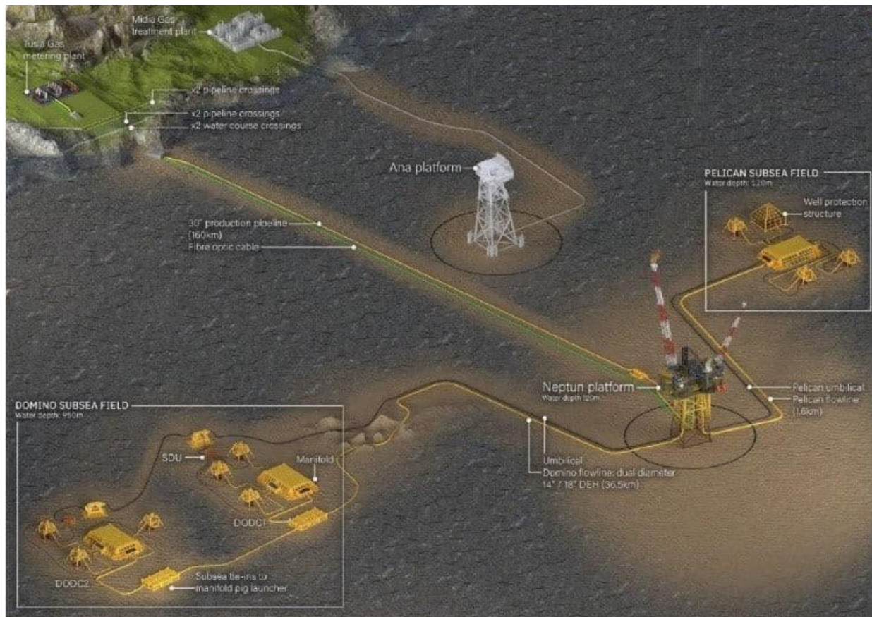
Figure 1 Schema of the Neptun Deep gas exploitation infrastructure
