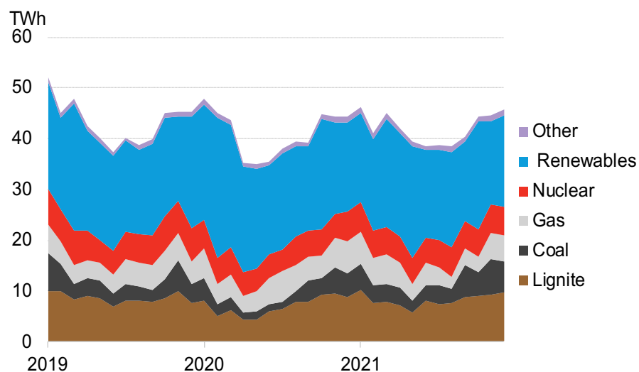
German power generation
