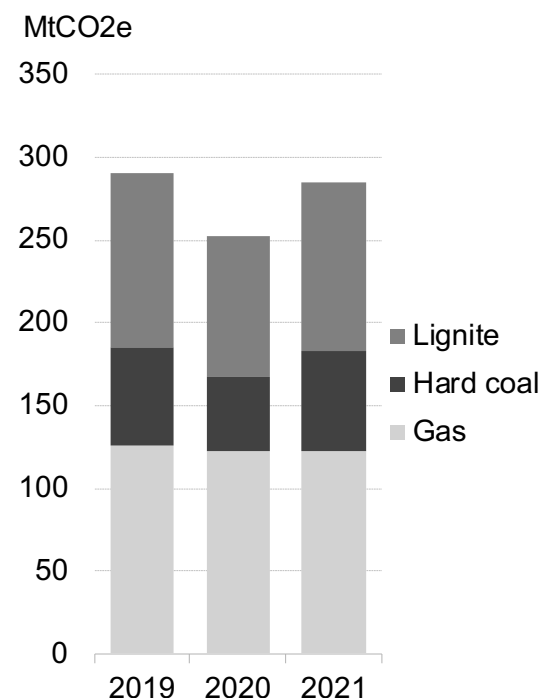
Emissions in Germany, Italy, France, U.K.
