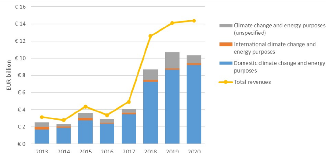
Auctioning revenues and reported usage (€Bn) – EU 27 Source : EU Climate Action Progress Report 2021
