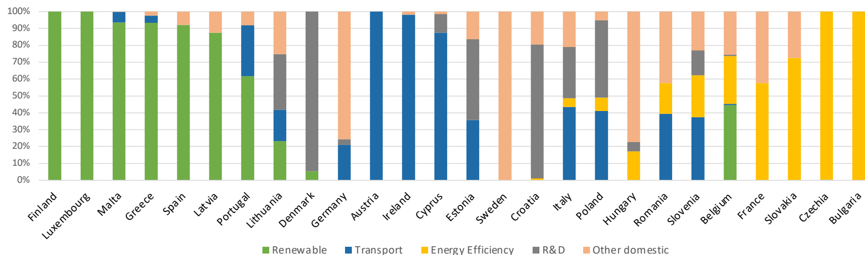
Self reported use of ETS auctioning revenues spent on climate change and energy in 2020 Data : Reportnet dataflows
