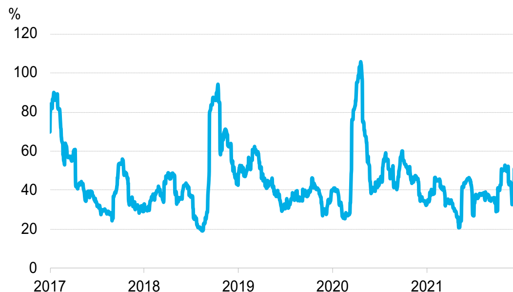
Volatility
